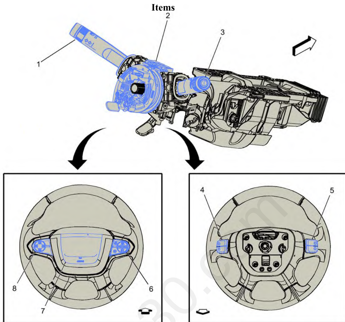
Fig. 5: Steering Column Components Courtesy of GENERAL MOTORS COMPANY
